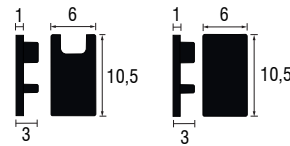
601T003F Tappi (opzionale) Terminals (optional) Verschlüsse (optional) 601T003CF Tappi chiusi (opzionale) Closed terminals (optional) Verschlüsse (optional)
